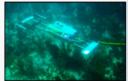
Underwater, an EM61 mounted on an ROV working above environmentally sensitive coral in Culebra, PR (USA)
